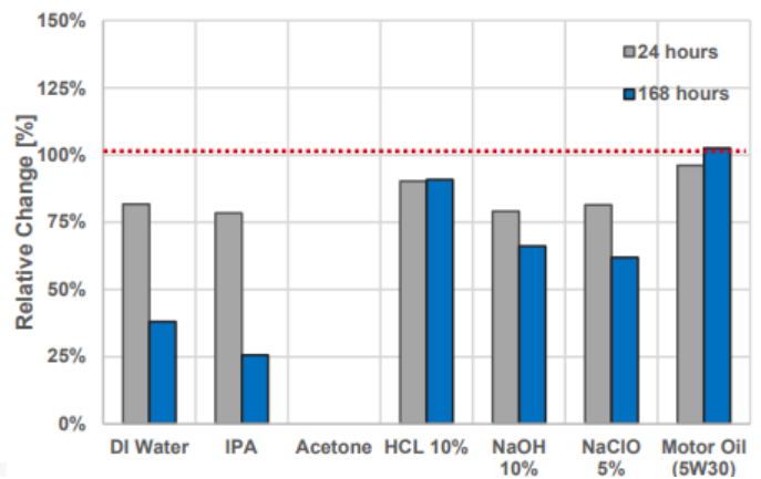
Stress at Yield after Immersion Time
