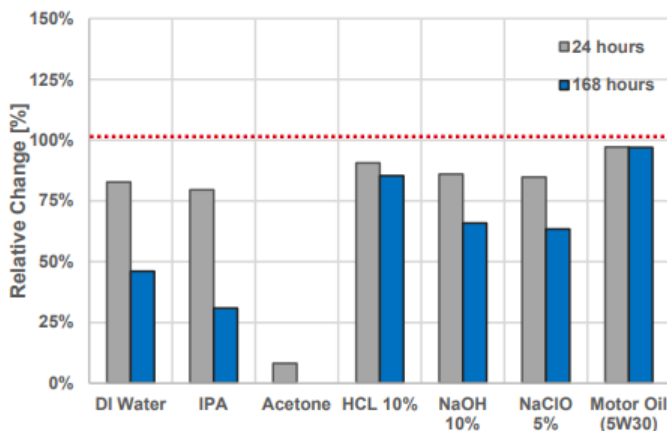
Stress at Break after Immersion Time
