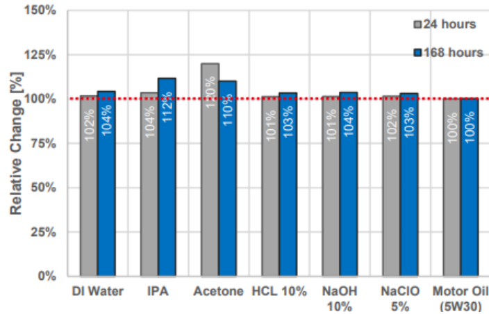
Mass Soak after Immersion Time
