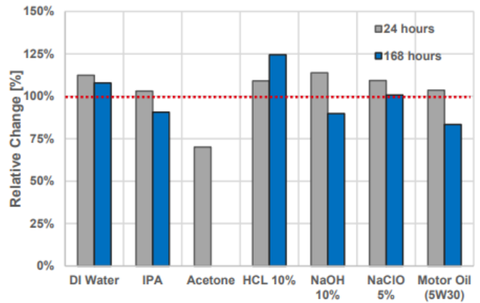
Elongation at Break after Immersion Time
