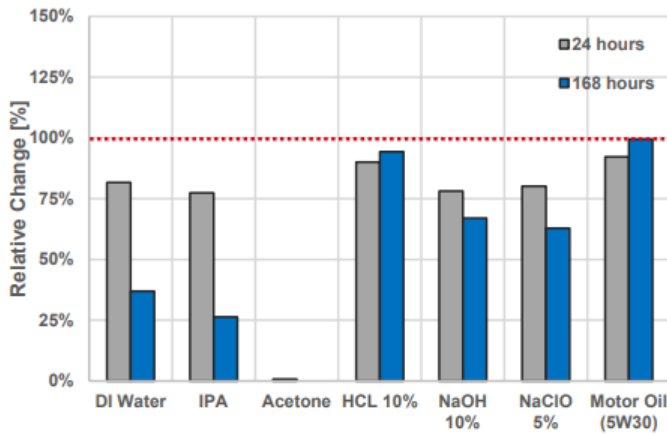
Young's Modulus after Immersion Time
